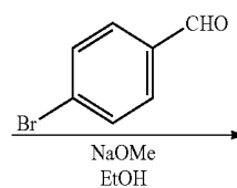
Compound 19
