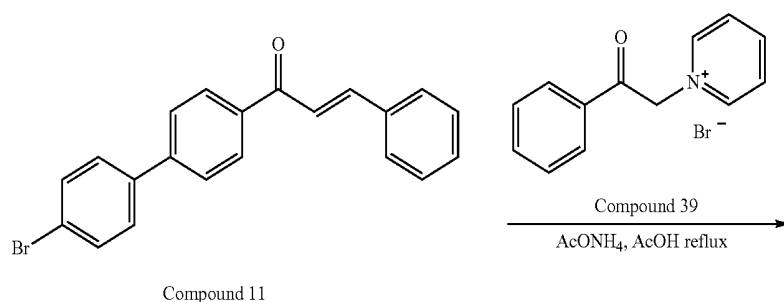
Compound 11
