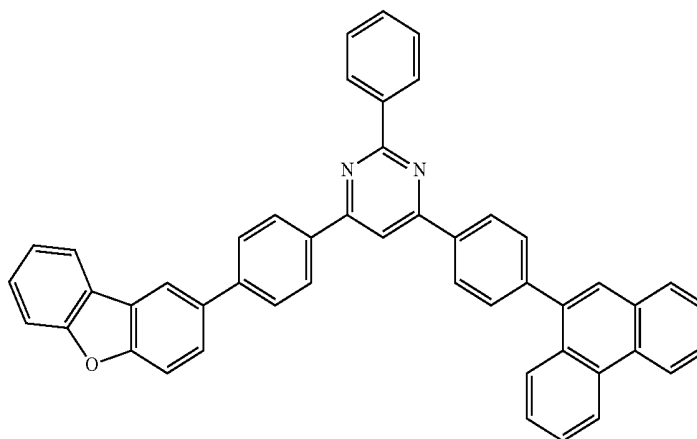
Compound 22
