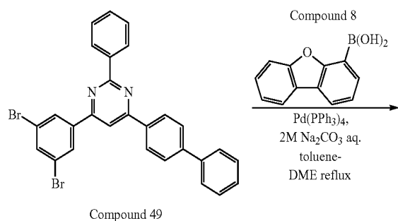
Compound 49
