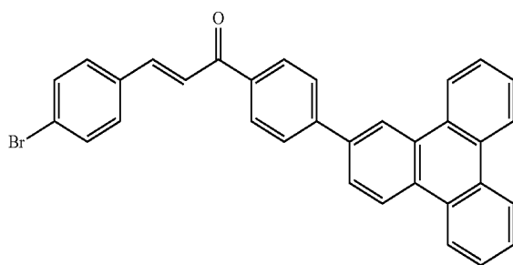
Compound 57
