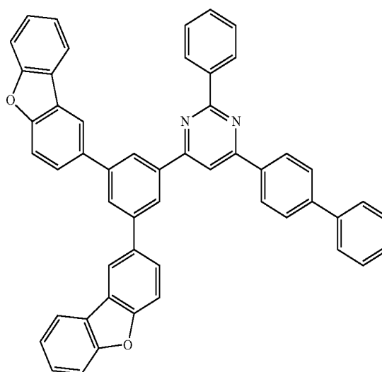
Compound 50
