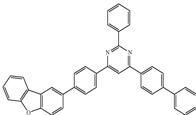
Compound 7
