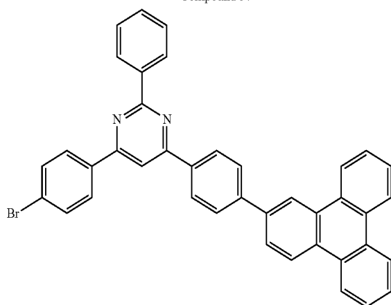
Compound 58
