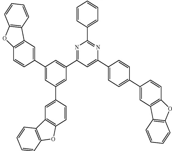
Compound 38
