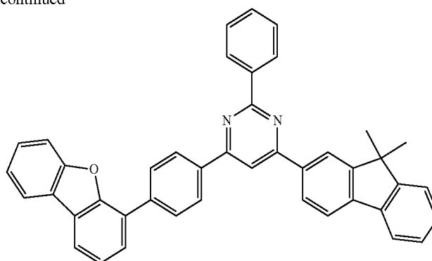
Compound 52
