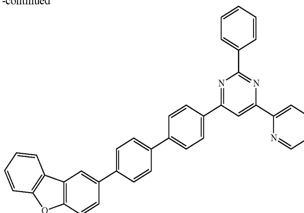
Compound 46
