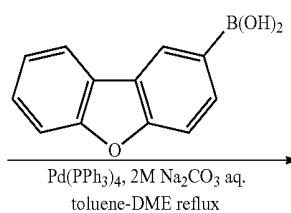
Compound 6
