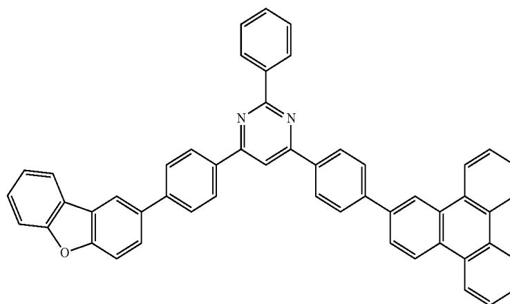
Compound 59
