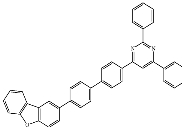
Compound 13
