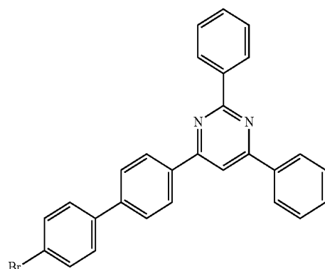
Compound 12
