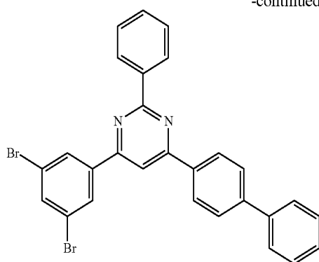
Compound 49
