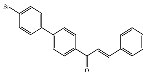
Compound 11
