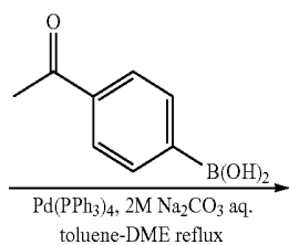
Compound 55
