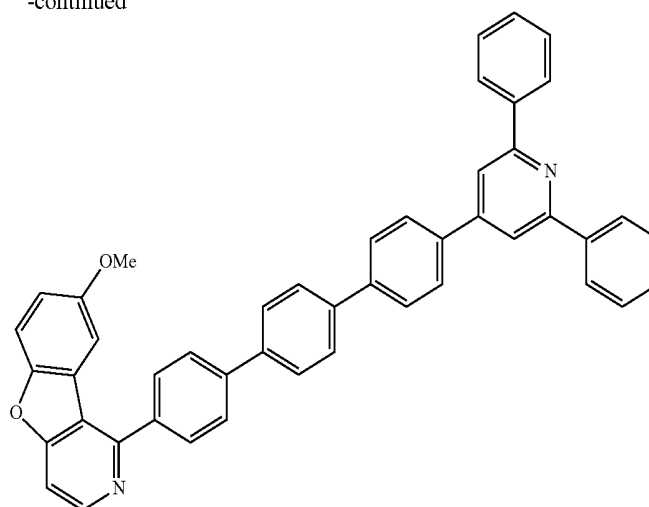
Compound 42
