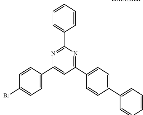
Compound 5
