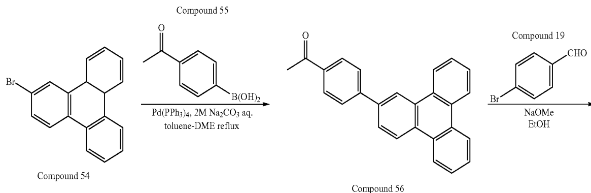
Compound 56
