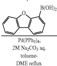
Compound 8
